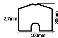
Eave Purlin
