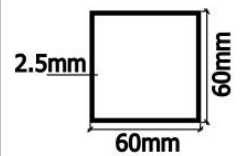
Roof Purlin
